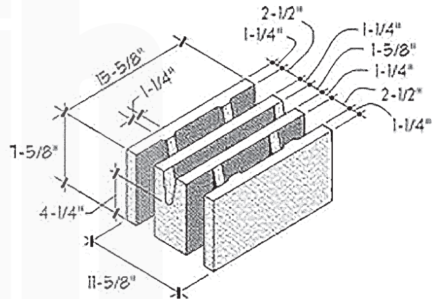
STRETCHER - 12 X 8 X 16
