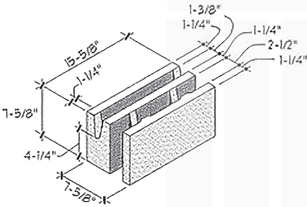
STRETCHER - 8 X 8 X 16
